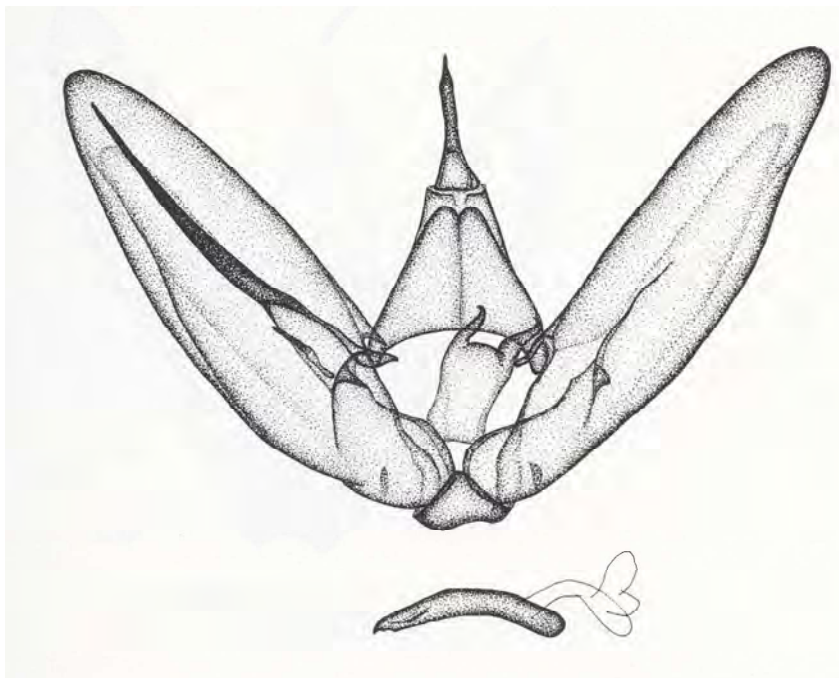
Male genitalia (after Arenberger, 1995)
