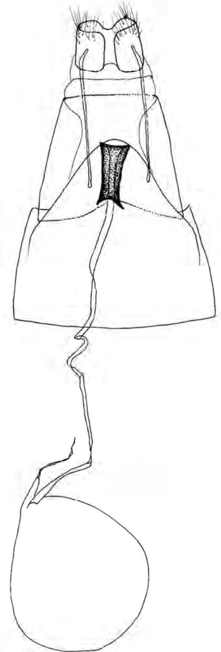
Female genitalia (After Arenberger, 2002)
