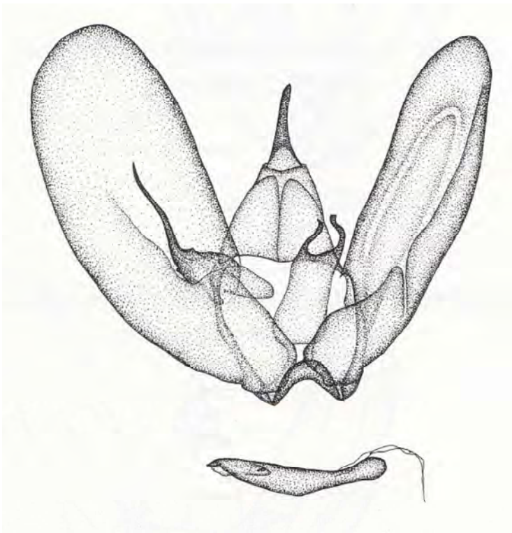
Male genitalia (after Arenberger, 1995)
