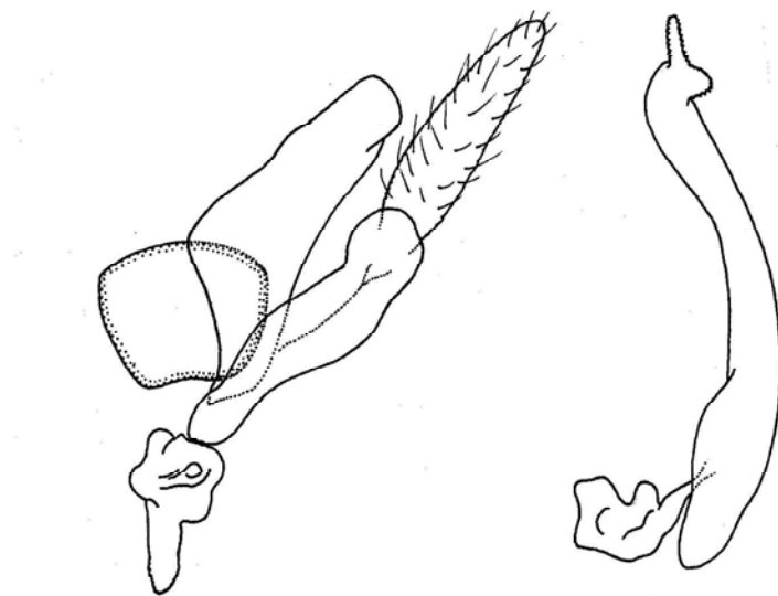
Male genitalia + aedeagus
