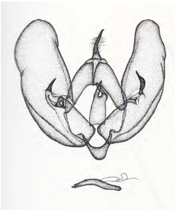
Male genitalia (after Arenberger, 1995)
