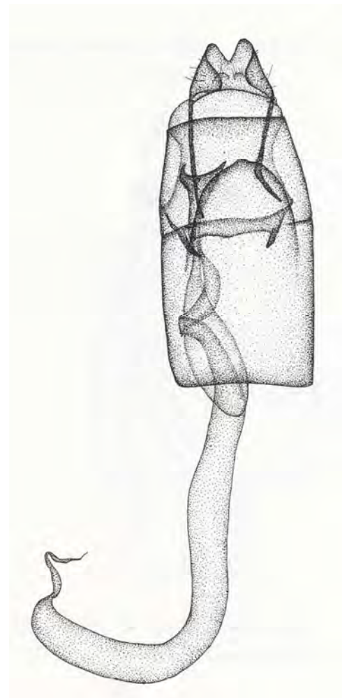
Female genitalia (after Arenberger, 1995)
