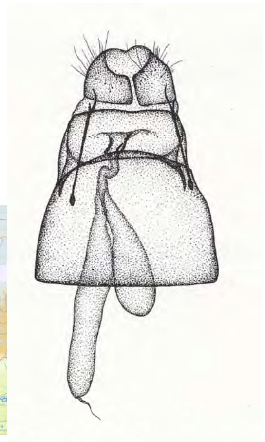
Female genitalia (after Arenberger, 1995)
