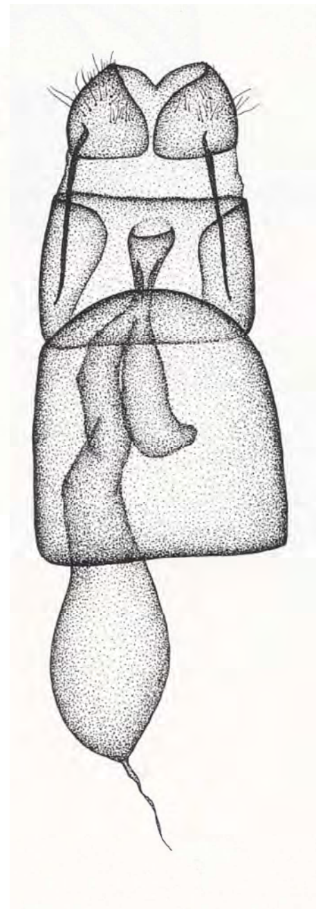
Female genitalia (after Arenberger, 1995)
