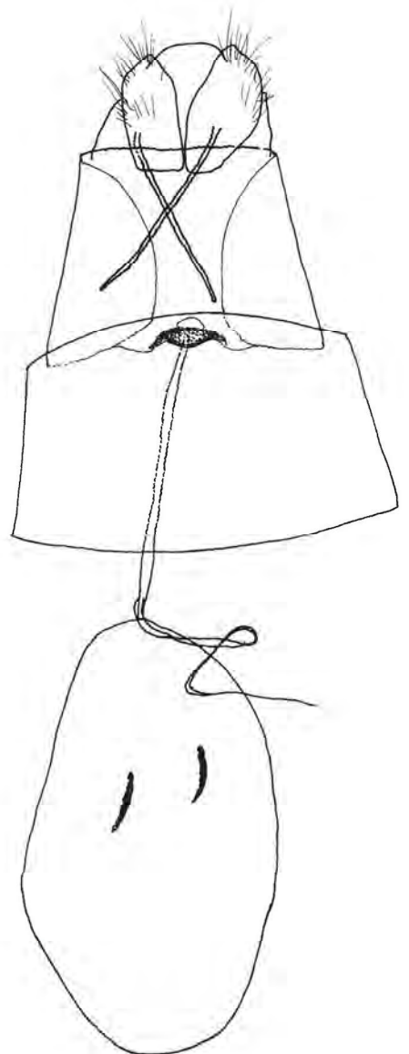
Female genitalia (After Arenberger, 2002)
