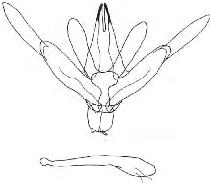
Male genitalia (After Arenberger, 2002)
