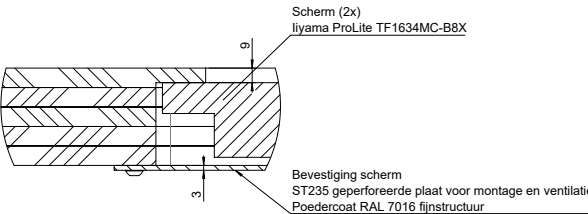
DETAIL C SCALE 1 : 2
